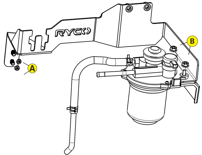
FIG. 2 BRACKET INSTALLATION
